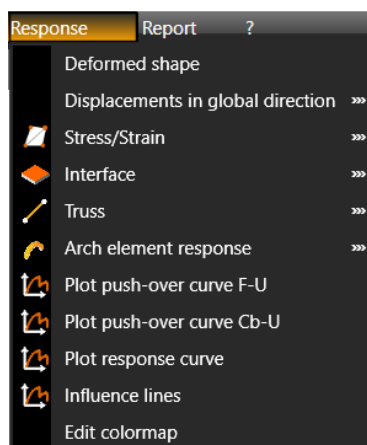
Figura 7.59 – Menu Response
