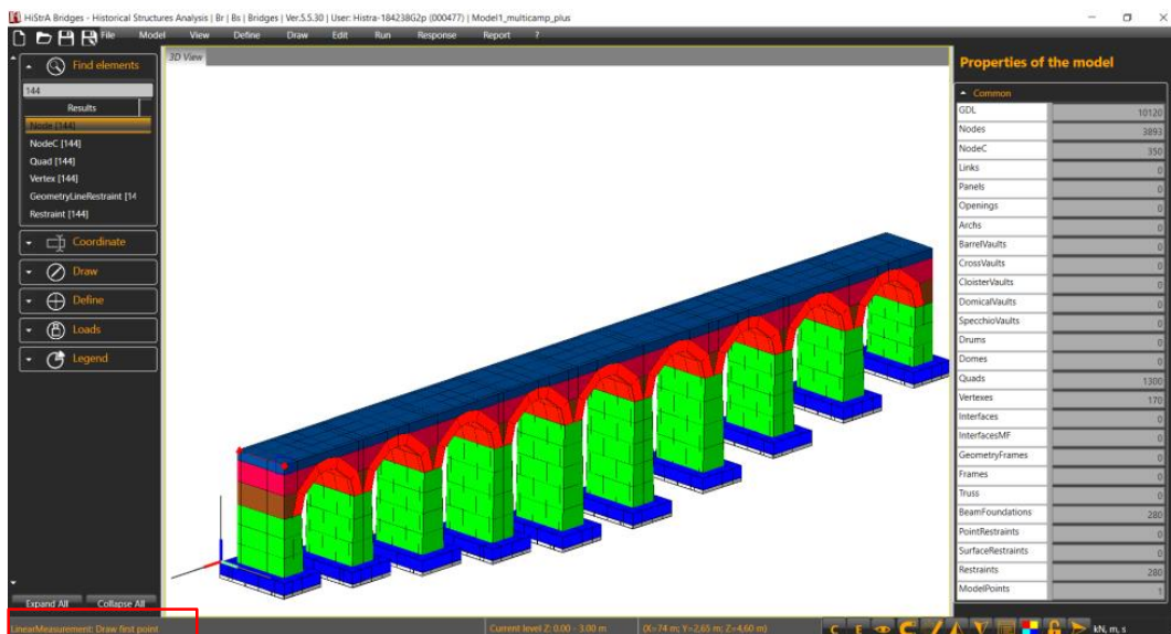
Figura 7.54– Edit > Distance
